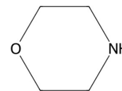
STRUCTURAL FORMULA
