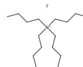
STRUCTURAL FORMULA
