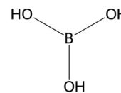
STRUCTURAL FORMULA
