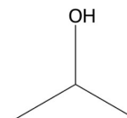
STRUCTURAL FORMULA
