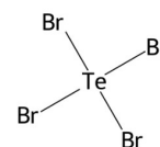
STRUCTURAL FORMULA
